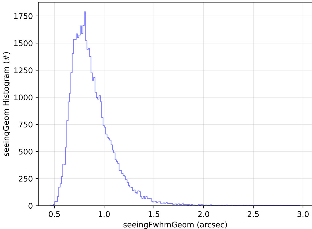
ddf_acor_sf20_lsf0_lsr0_v3.4_10yrs Yr 1 y band: seeingGeom Histogram
