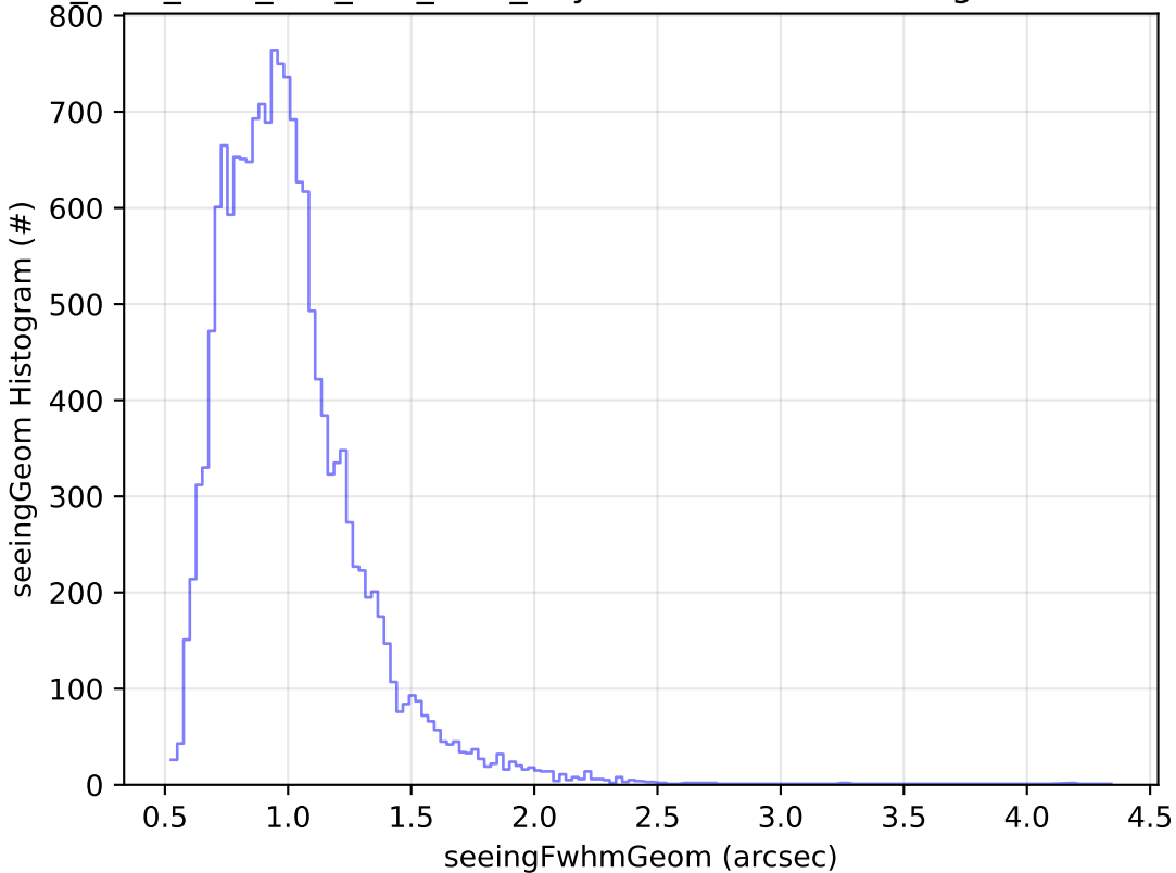
ddf_acor_sf20_lsf0_lsr0_v3.4_10yrs Yr 1 u band: seeingGeom Histogram
