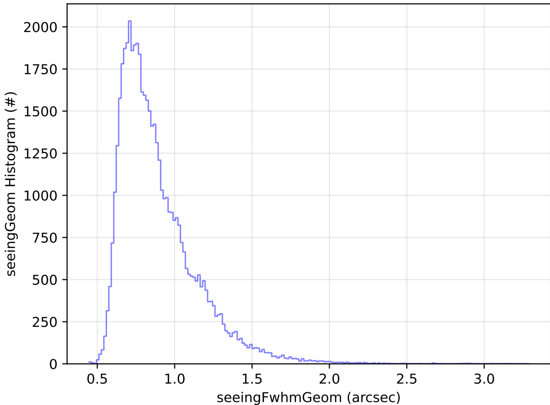
ddf_acor_sf20_lsf0_lsr0_v3.4_10yrs Yr 1 r band: seeingGeom Histogram
