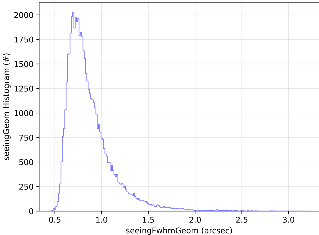
ddf_acor_sf20_lsf0_lsr0_v3.4_10yrs Yr 1 i band: seeingGeom Histogram
