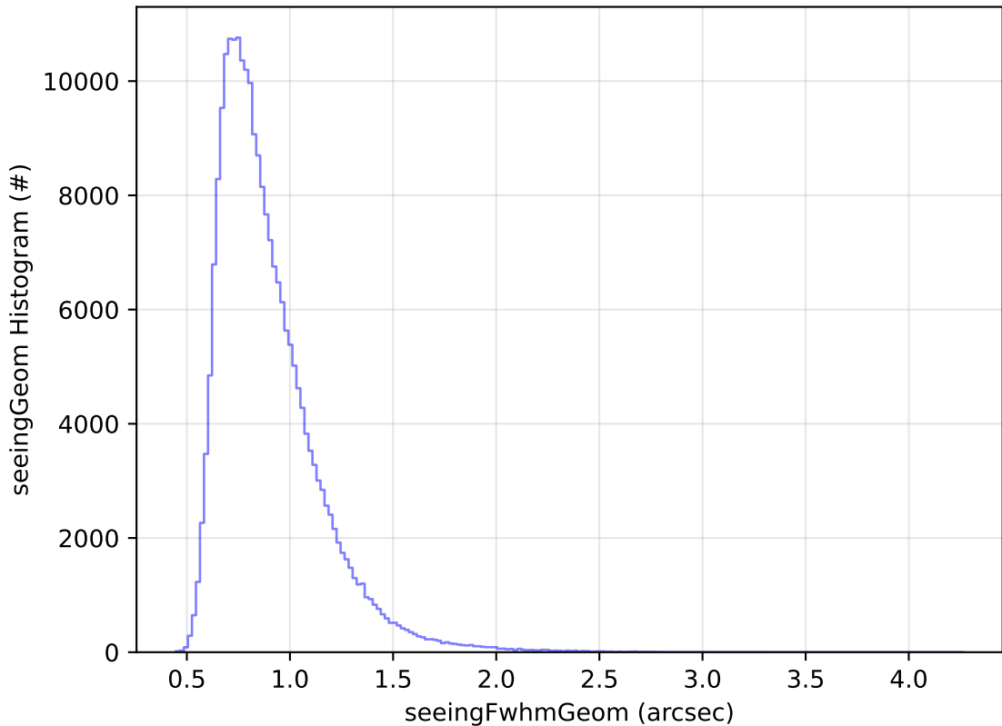
ddf_acor_sf20_lsf0_lsr0_v3.4_10yrs Yr 1 all bands: seeingGeom Histogram
