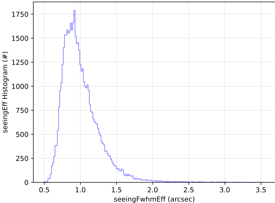
ddf_acor_sf20_lsf0_lsr0_v3.4_10yrs Yr 1 y band: seeingEff Histogram
