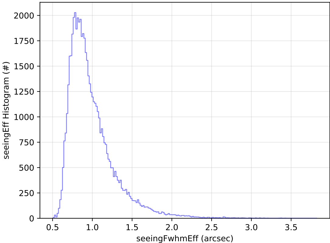
ddf_acor_sf20_lsf0_lsr0_v3.4_10yrs Yr 1 i band: seeingEff Histogram
