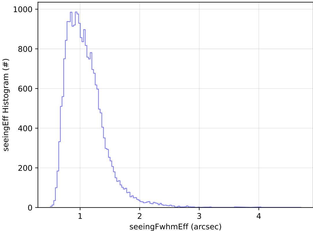
ddf_acor_sf20_lsf0_lsr0_v3.4_10yrs Yr 1 g band: seeingEff Histogram
