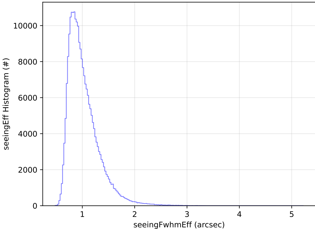
ddf_acor_sf20_lsf0_lsr0_v3.4_10yrs Yr 1 all bands: seeingEff Histogram
