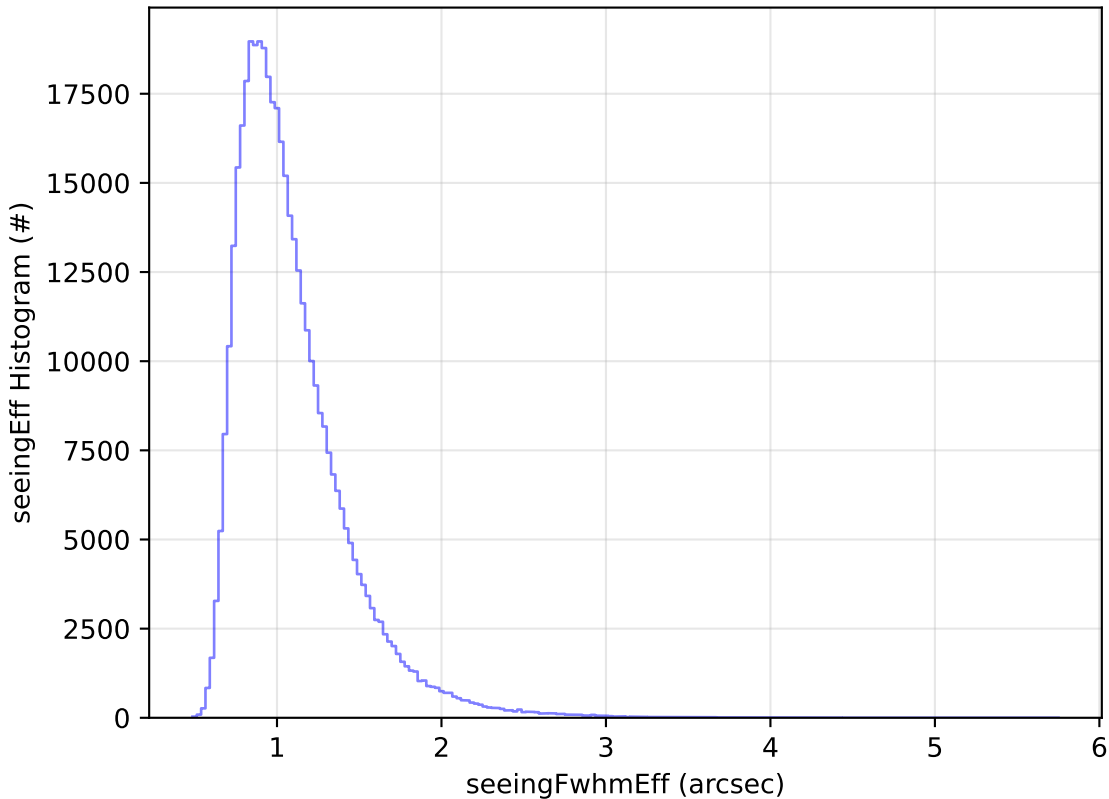
ddf_acor_sf20_lsf0_lsr0_v3.4_10yrs WFD z band: seeingEff Histogram
