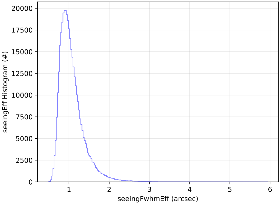
ddf_acor_sf20_lsf0_lsr0_v3.4_10yrs WFD y band: seeingEff Histogram
