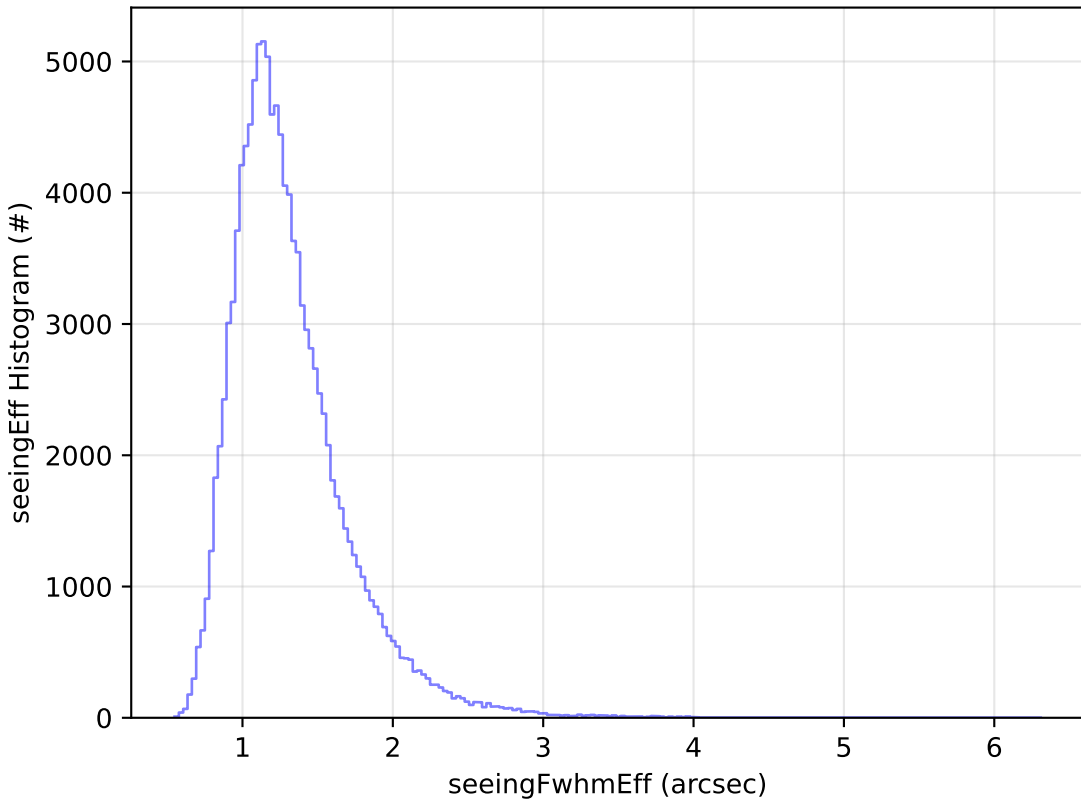
ddf_acor_sf20_lsf0_lsr0_v3.4_10yrs WFD u band: seeingEff Histogram
