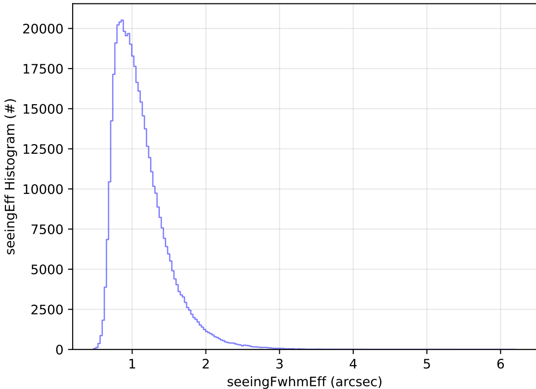
ddf_acor_sf20_lsf0_lsr0_v3.4_10yrs WFD r band: seeingEff Histogram
