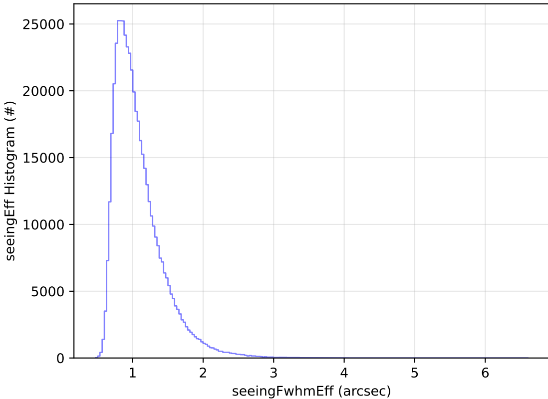
ddf_acor_sf20_lsf0_lsr0_v3.4_10yrs WFD i band: seeingEff Histogram
