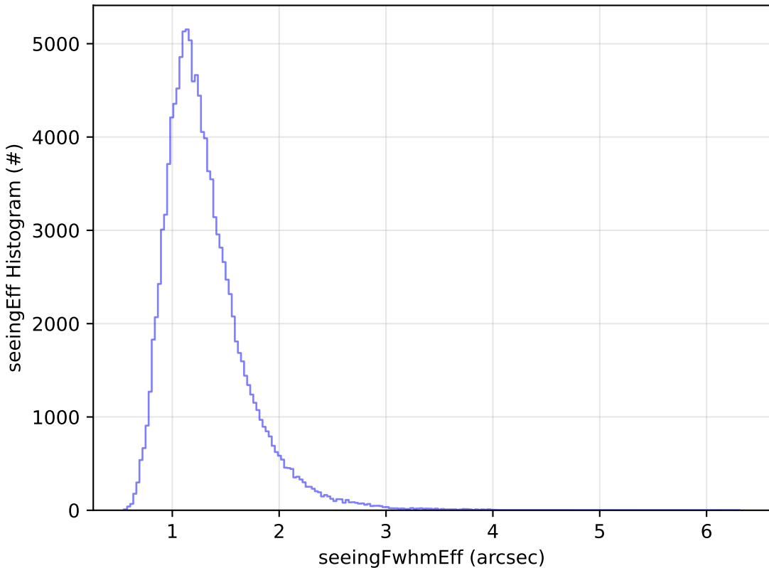
ddf_acor_sf20_lsf0_lsr0_v3.4_10yrs All sky u band: seeingEff Histogram
