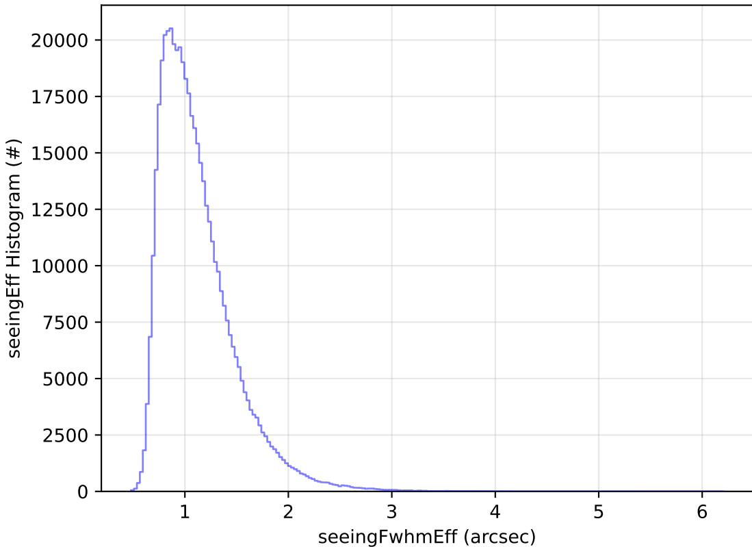
ddf_acor_sf20_lsf0_lsr0_v3.4_10yrs All sky r band: seeingEff Histogram
