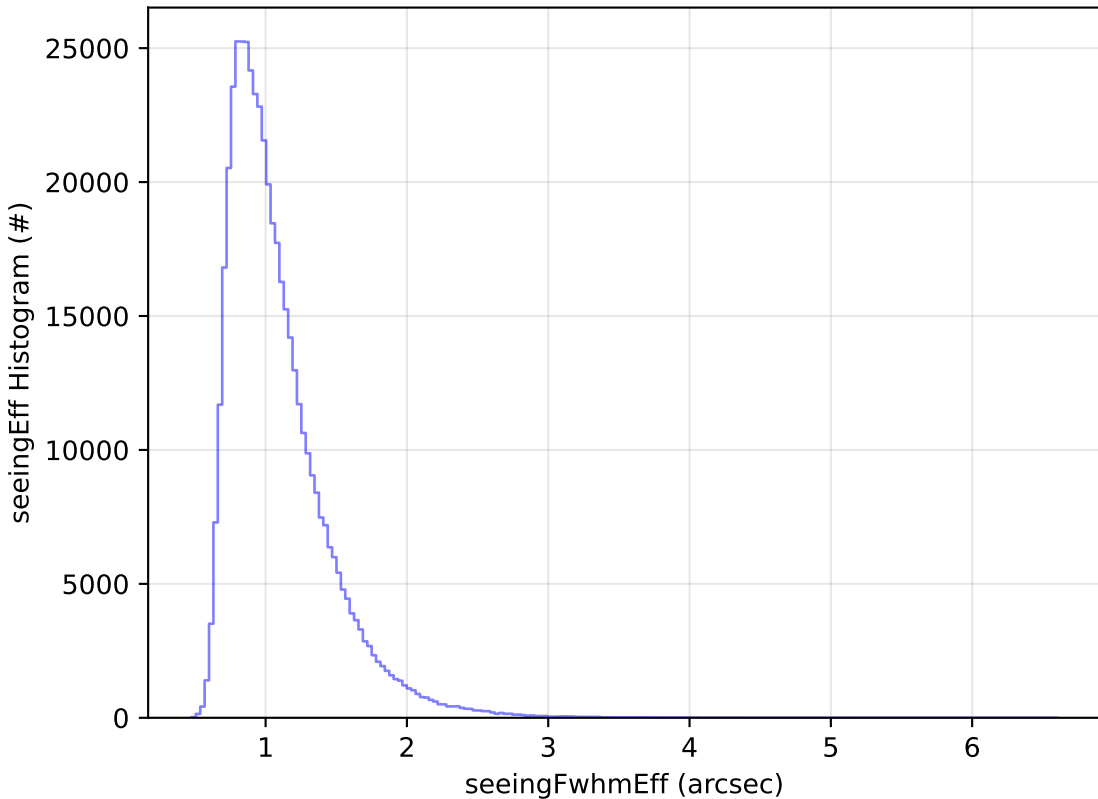
ddf_acor_sf20_lsf0_lsr0_v3.4_10yrs All sky i band: seeingEff Histogram
