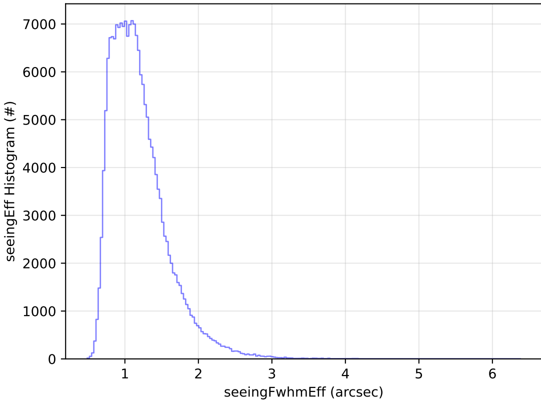
ddf_acor_sf20_lsf0_lsr0_v3.4_10yrs All sky g band: seeingEff Histogram
