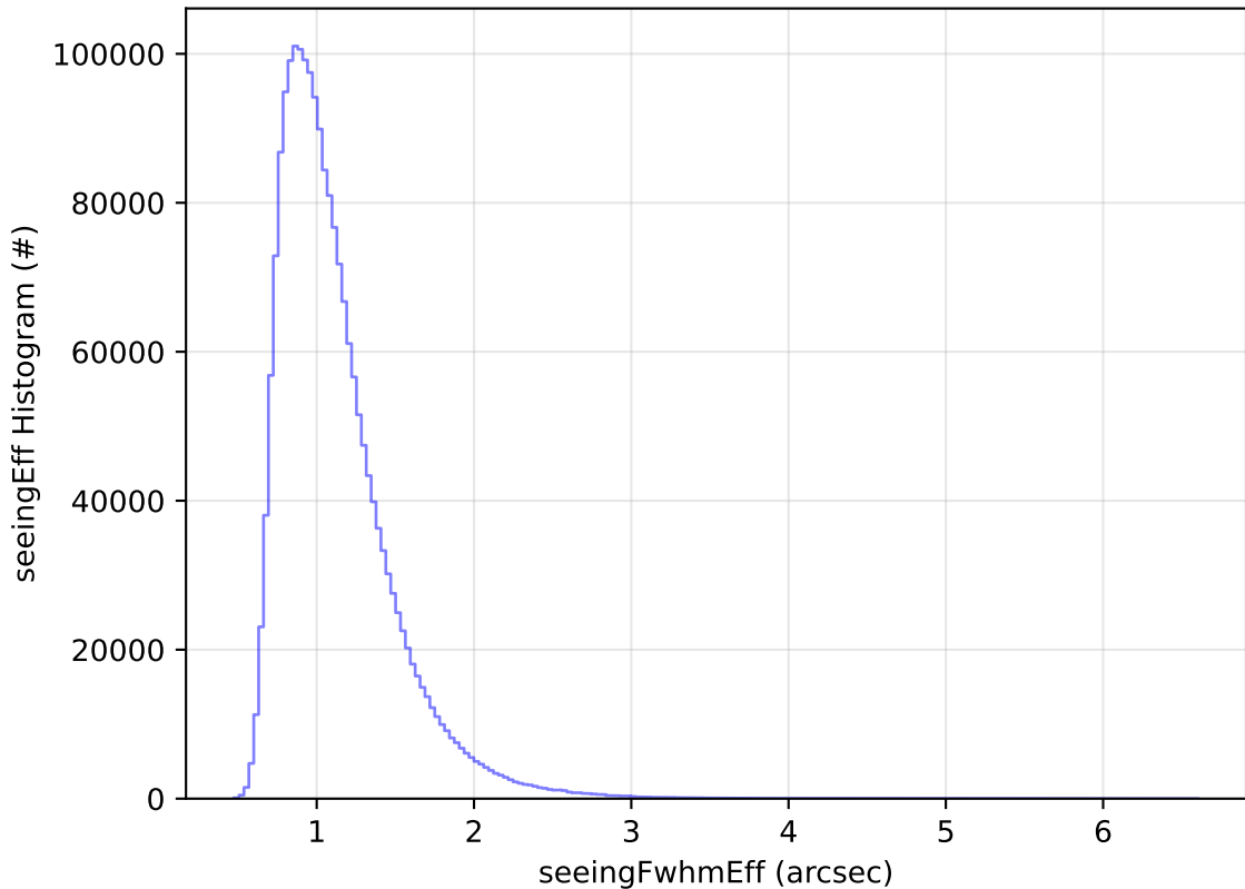
ddf_acor_sf20_lsf0_lsr0_v3.4_10yrs All sky all bands: seeingEff Histogram
