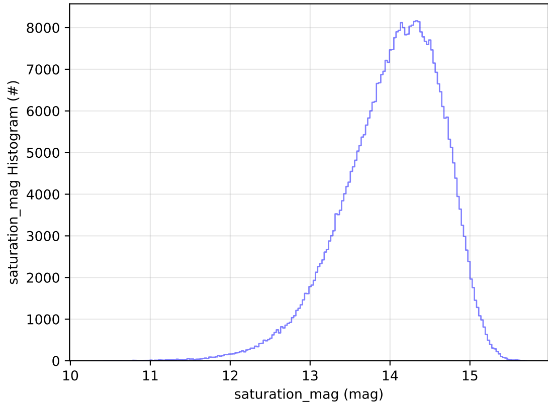
ddf_acor_sf20_lsf0_lsr0_v3.4_10yrs WFD z band: saturation_mag Histogram
