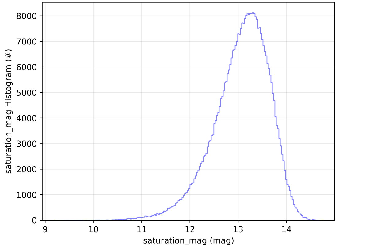
ddf_acor_sf20_lsf0_lsr0_v3.4_10yrs WFD y band: saturation_mag Histogram
