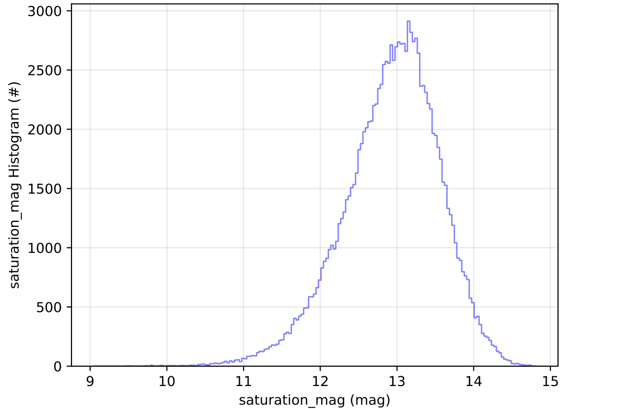
ddf_acor_sf20_lsf0_lsr0_v3.4_10yrs WFD u band: saturation_mag Histogram
