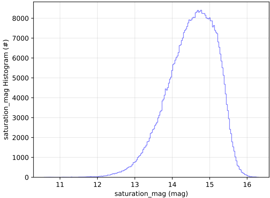
ddf_acor_sf20_lsf0_lsr0_v3.4_10yrs WFD r band: saturation_mag Histogram
