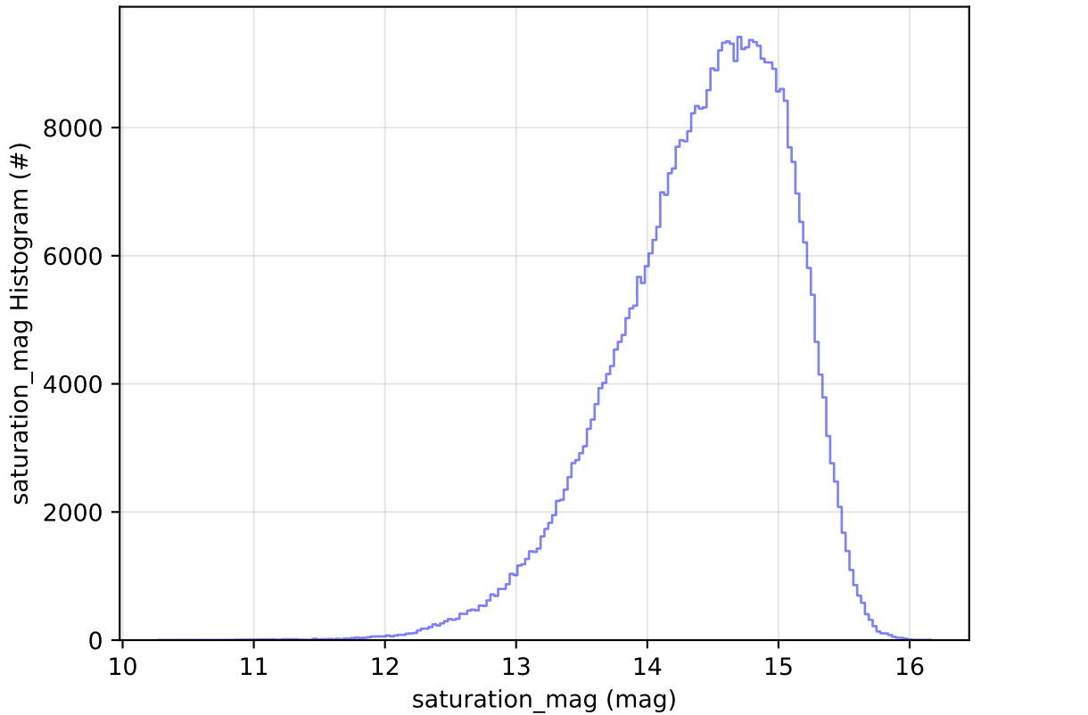
ddf_acor_sf20_lsf0_lsr0_v3.4_10yrs WFD i band: saturation_mag Histogram
