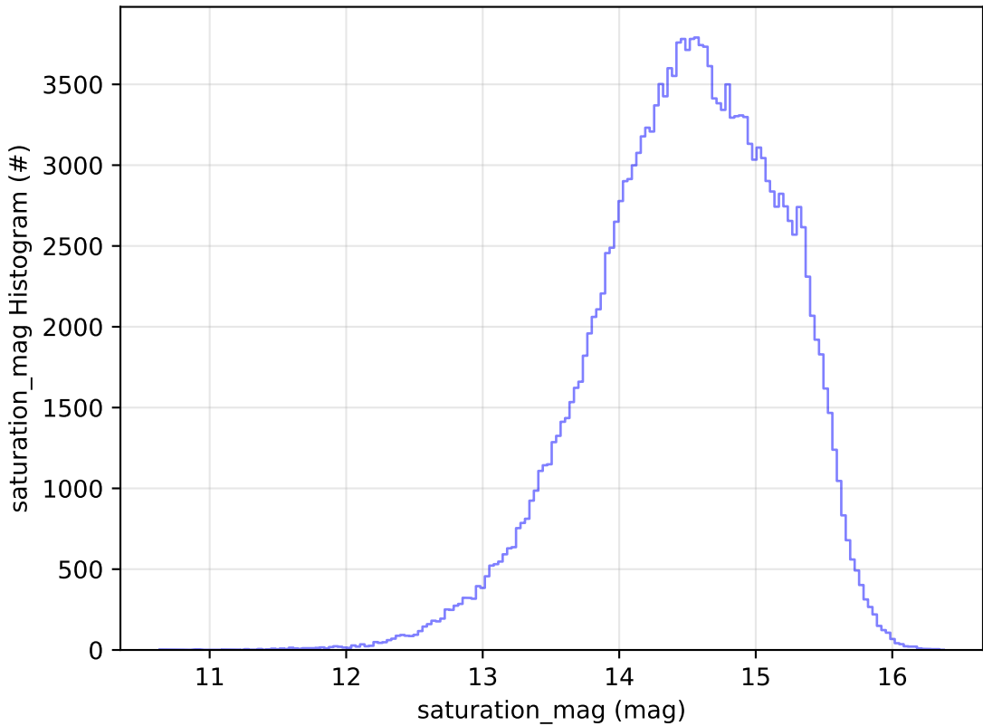
ddf_acor_sf20_lsf0_lsr0_v3.4_10yrs WFD g band: saturation_mag Histogram
