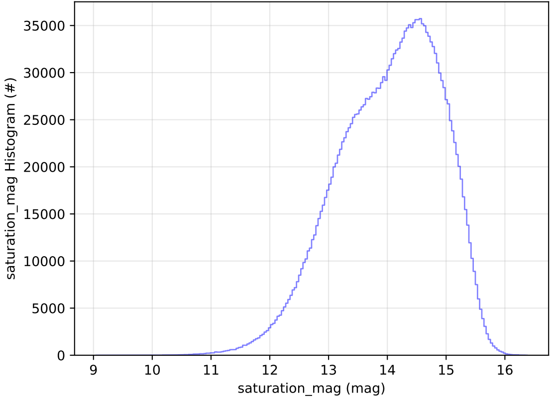
ddf_acor_sf20_lsf0_lsr0_v3.4_10yrs WFD all bands: saturation_mag Histogram
