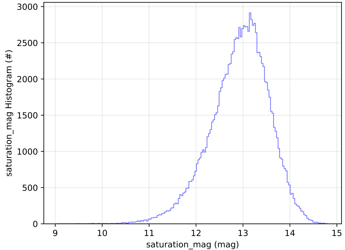
ddf_acor_sf20_lsf0_lsr0_v3.4_10yrs All sky u band: saturation_mag Histogram
