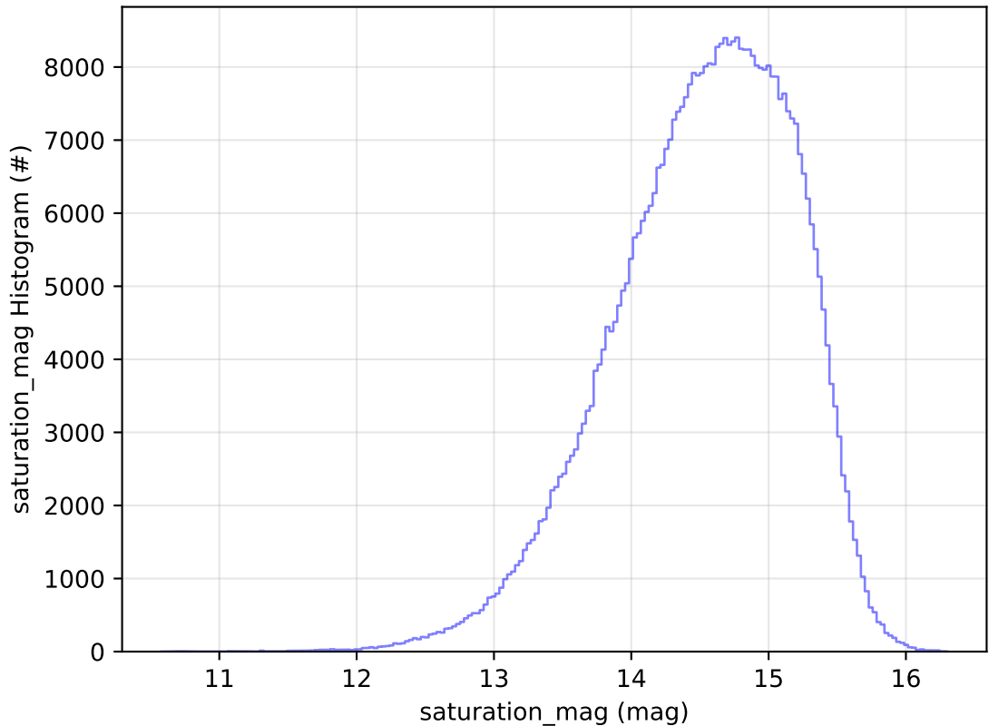
ddf_acor_sf20_lsf0_lsr0_v3.4_10yrs All sky r band: saturation_mag Histogram
