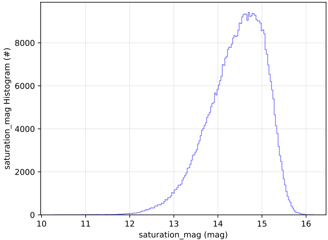
ddf_acor_sf20_lsf0_lsr0_v3.4_10yrs All sky i band: saturation_mag Histogram
