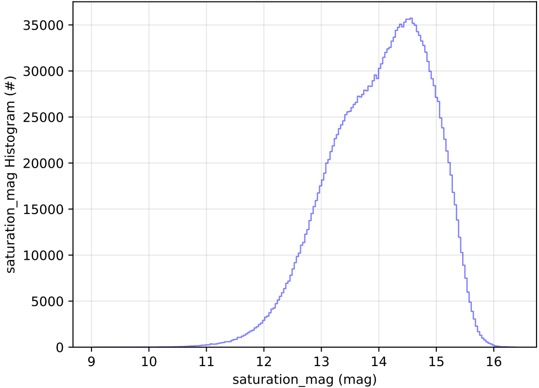
ddf_acor_sf20_lsf0_lsr0_v3.4_10yrs All sky all bands: saturation_mag Histogram
