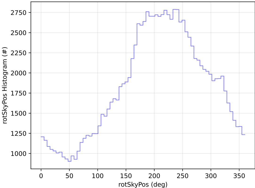
ddf_acor_sf20_lsf0_lsr0_v3.4_10yrs WFD u band: rotSkyPos Histogram
