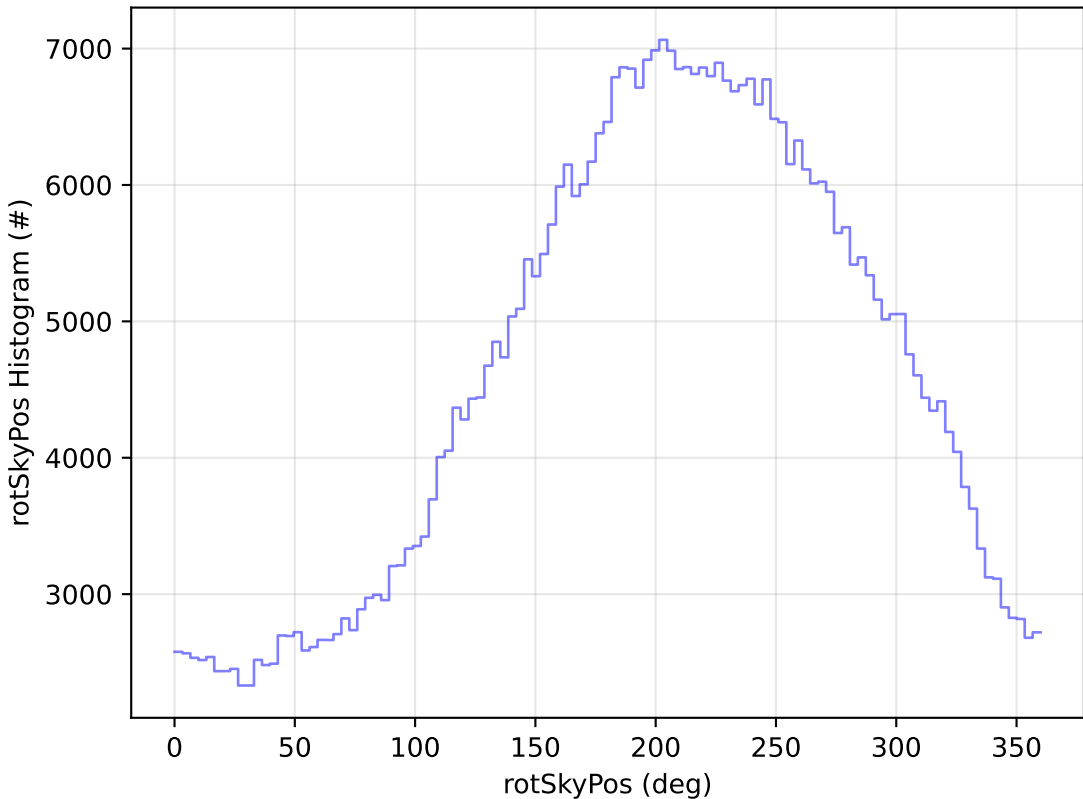
ddf_acor_sf20_lsf0_lsr0_v3.4_10yrs WFD i band: rotSkyPos Histogram
