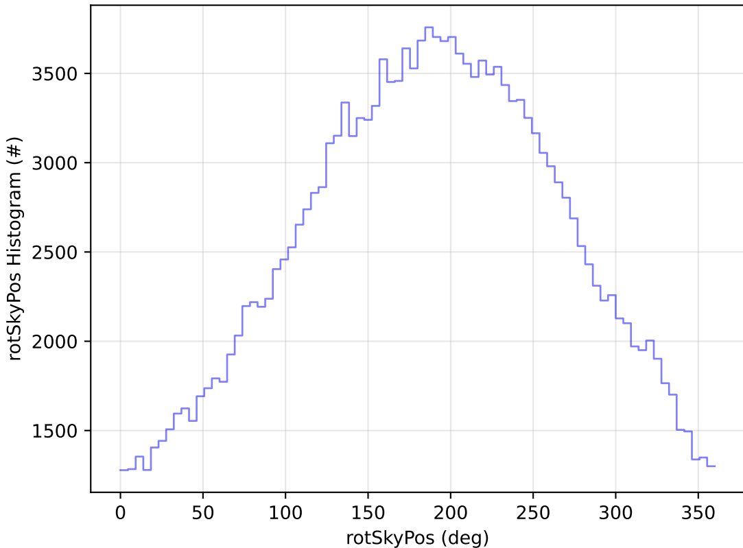
ddf_acor_sf20_lsf0_lsr0_v3.4_10yrs WFD g band: rotSkyPos Histogram
