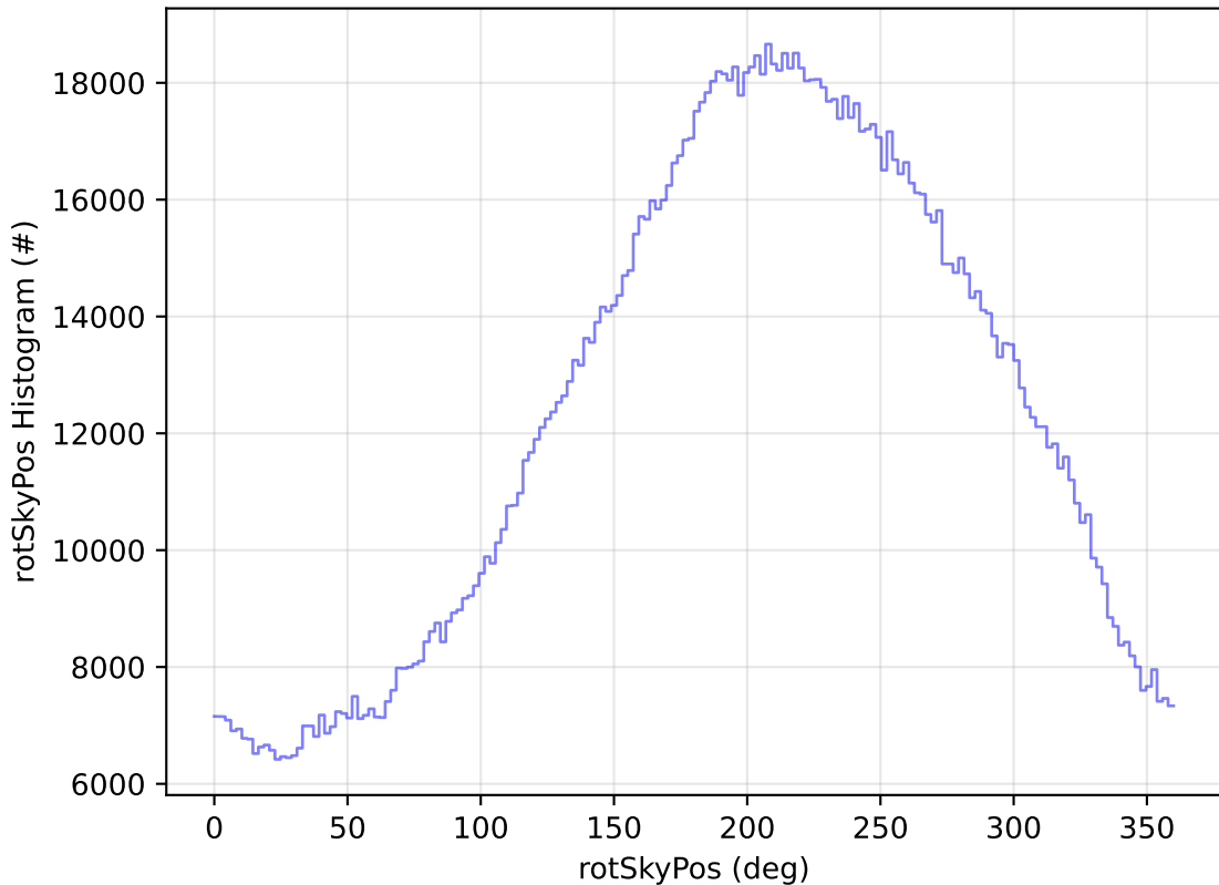
ddf_acor_sf20_lsf0_lsr0_v3.4_10yrs WFD all bands: rotSkyPos Histogram
