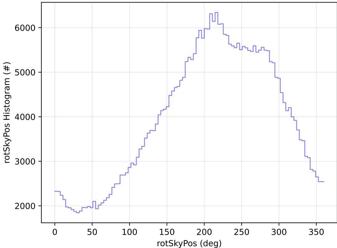
ddf_acor_sf20_lsf0_lsr0_v3.4_10yrs All sky y band: rotSkyPos Histogram
