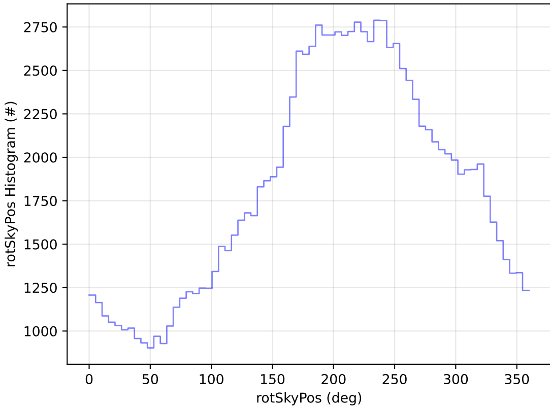
ddf_acor_sf20_lsf0_lsr0_v3.4_10yrs All sky u band: rotSkyPos Histogram
