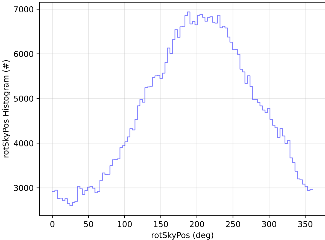
ddf_acor_sf20_lsf0_lsr0_v3.4_10yrs All sky r band: rotSkyPos Histogram
