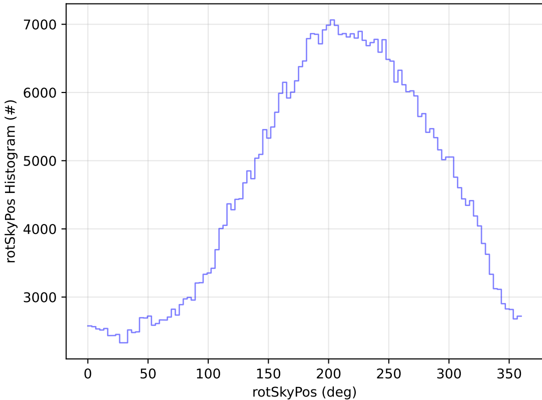
ddf_acor_sf20_lsf0_lsr0_v3.4_10yrs All sky i band: rotSkyPos Histogram
