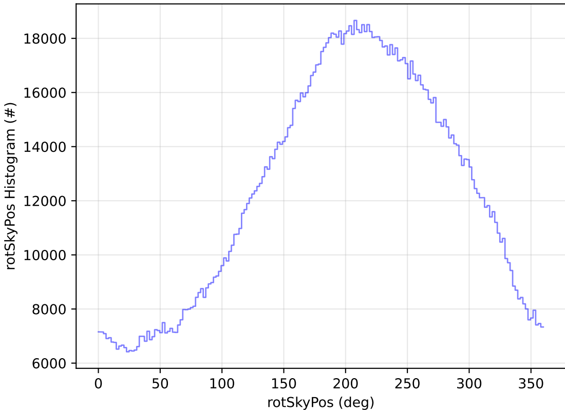
ddf_acor_sf20_lsf0_lsr0_v3.4_10yrs All sky all bands: rotSkyPos Histogram
