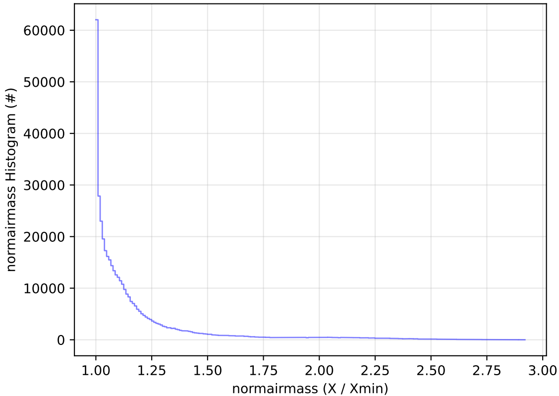
ddf_acor_sf20_lsf0_lsr0_v3.4_10yrs WFD z band: normairmass Histogram
