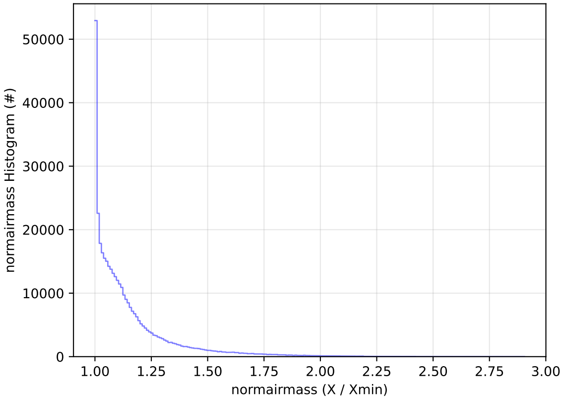
ddf_acor_sf20_lsf0_lsr0_v3.4_10yrs WFD y band: normairmass Histogram
