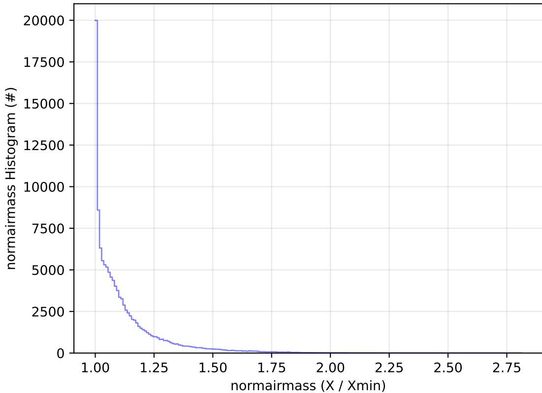
ddf_acor_sf20_lsf0_lsr0_v3.4_10yrs WFD u band: normairmass Histogram
