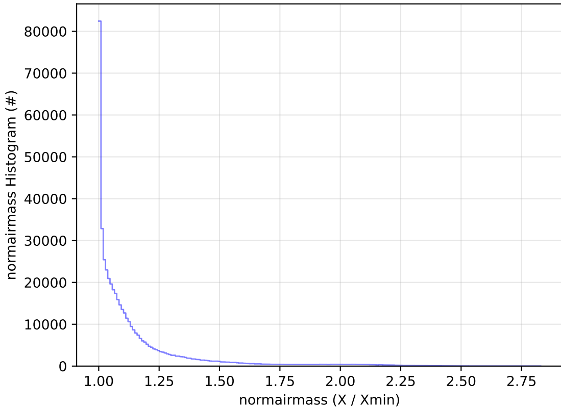
ddf_acor_sf20_lsf0_lsr0_v3.4_10yrs WFD r band: normairmass Histogram
