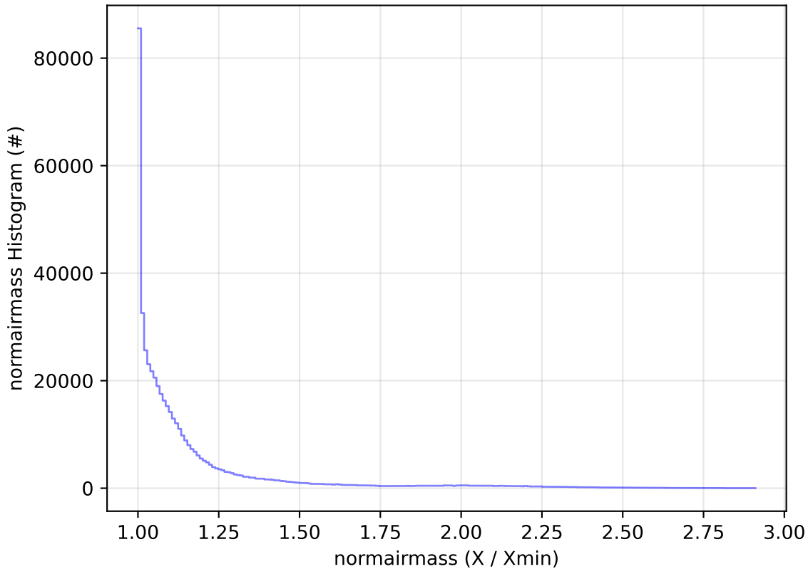
ddf_acor_sf20_lsf0_lsr0_v3.4_10yrs WFD i band: normairmass Histogram
