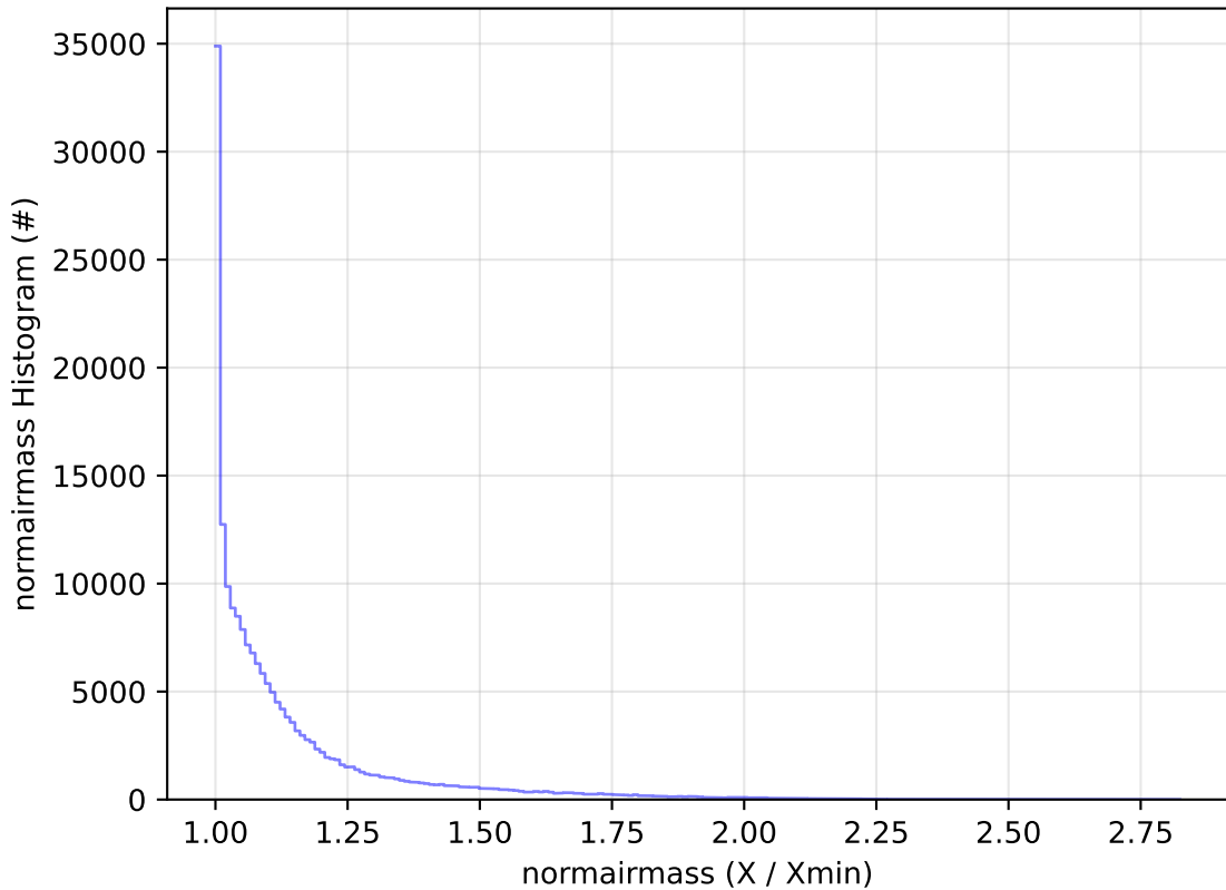
ddf_acor_sf20_lsf0_lsr0_v3.4_10yrs WFD g band: normairmass Histogram
