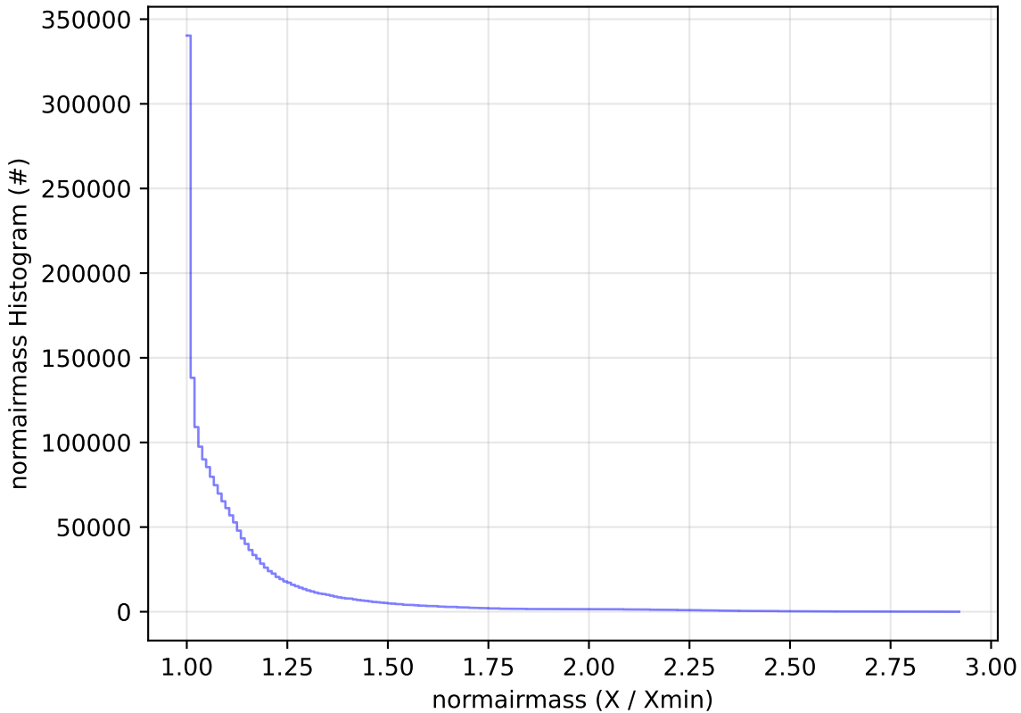
ddf_acor_sf20_lsf0_lsr0_v3.4_10yrs WFD all bands: normairmass Histogram
