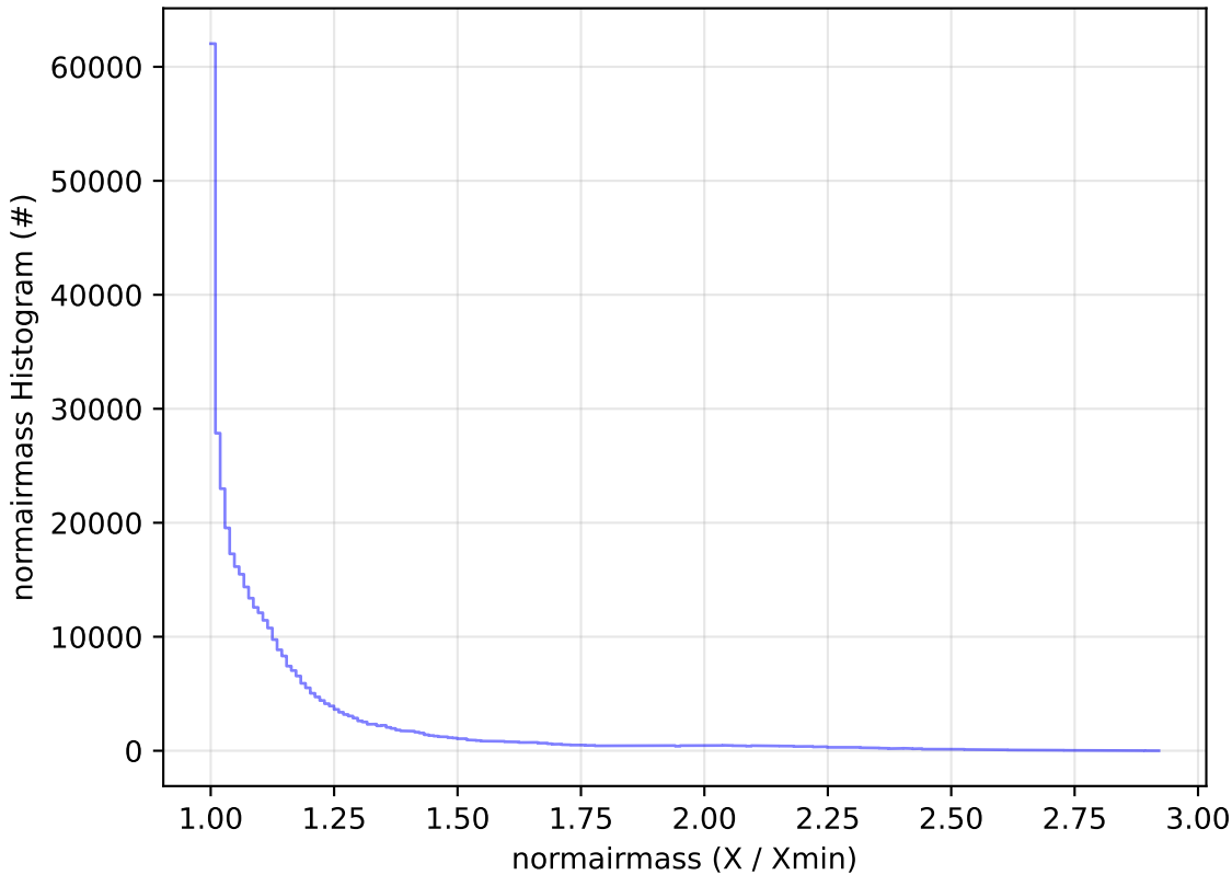
ddf_acor_sf20_lsf0_lsr0_v3.4_10yrs All sky z band: normairmass Histogram
