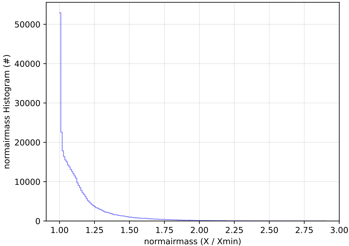
ddf_acor_sf20_lsf0_lsr0_v3.4_10yrs All sky y band: normairmass Histogram
