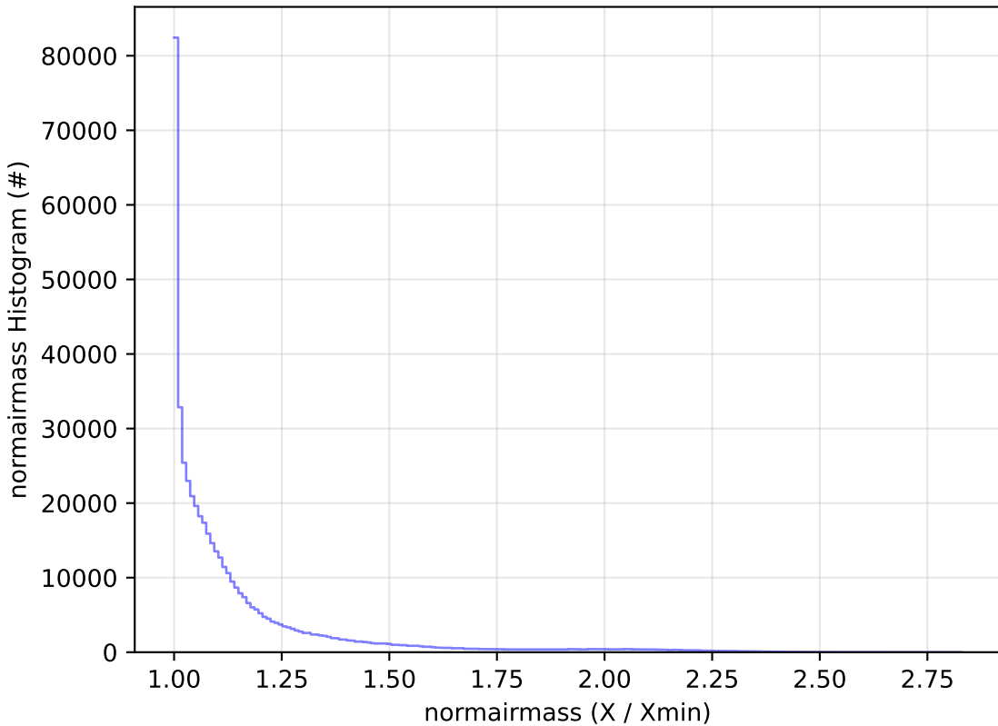
ddf_acor_sf20_lsf0_lsr0_v3.4_10yrs All sky r band: normairmass Histogram
