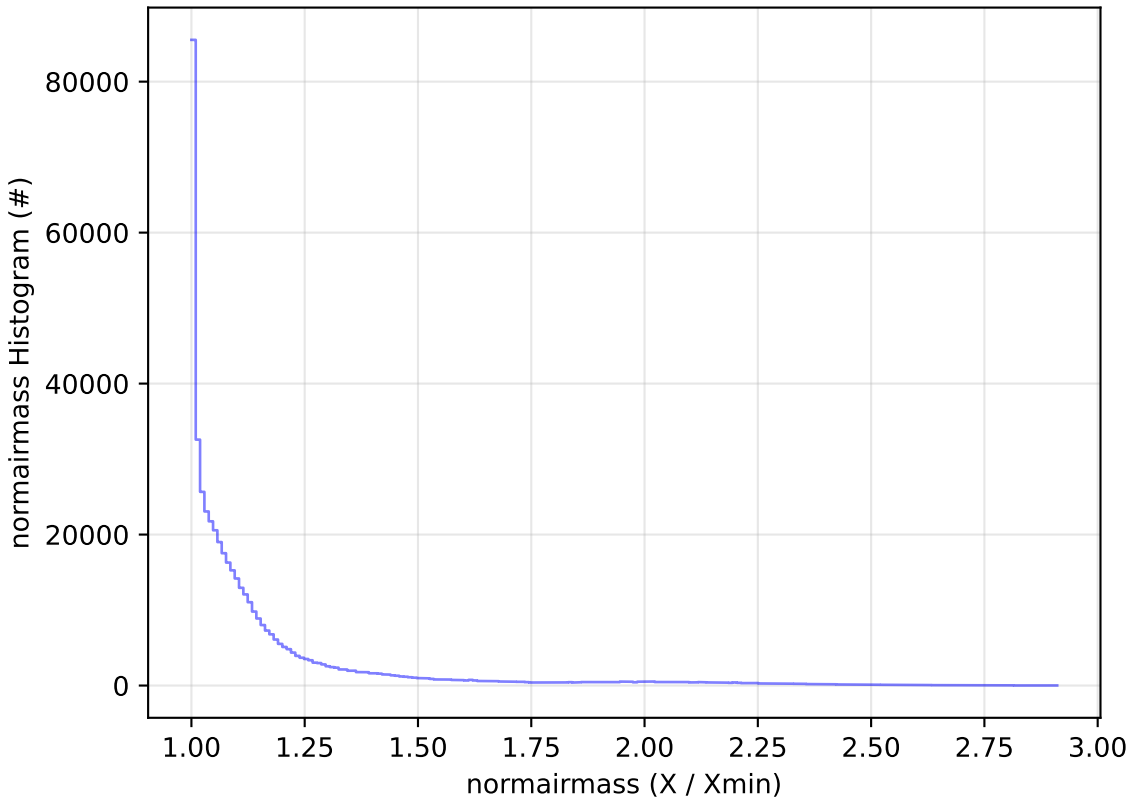
ddf_acor_sf20_lsf0_lsr0_v3.4_10yrs All sky i band: normairmass Histogram
